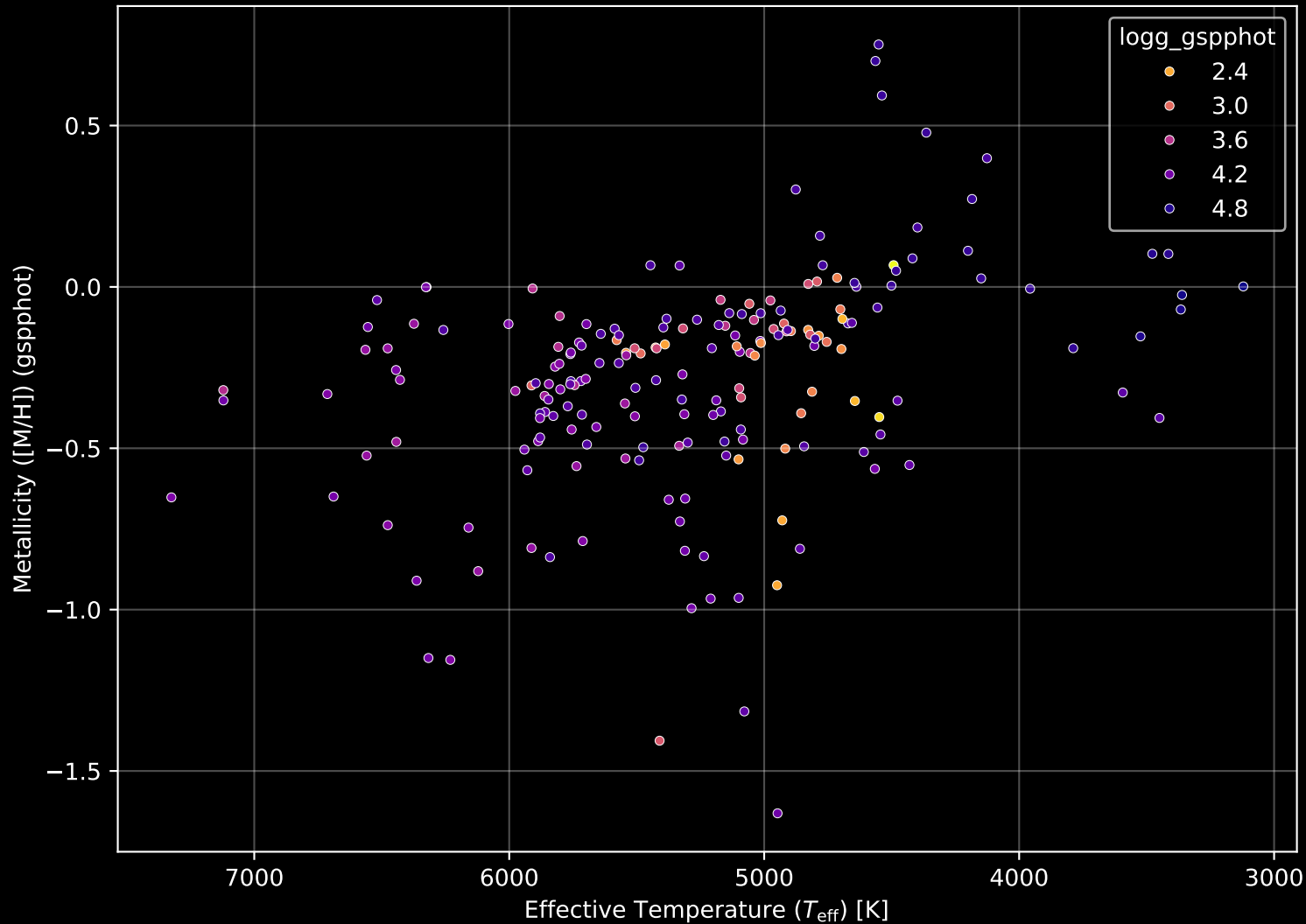
APOGEE DR17 Field: [176-27-O] Stellar Population Parameters (n= 196)
