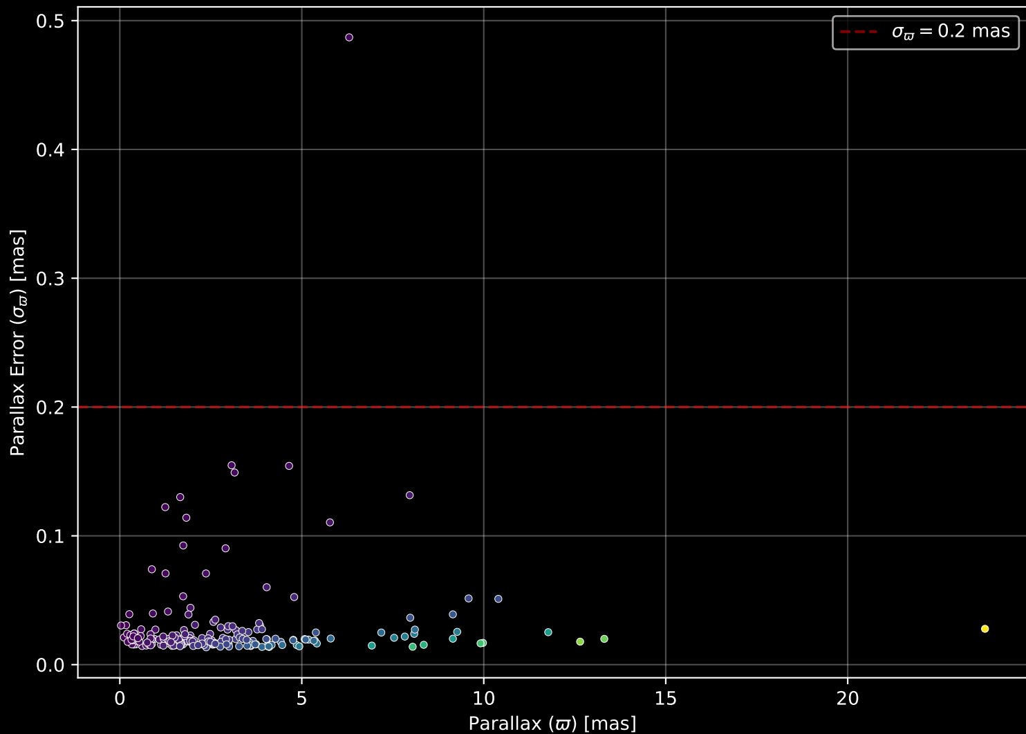
APOGEE DR17 Field: [176-27-O] Parallax Quality (n= 196)
