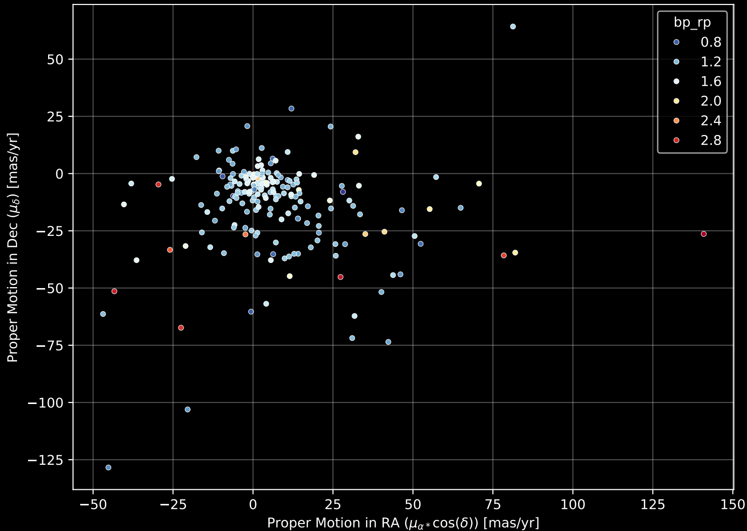
APOGEE DR17 Field: [176-27-O] Proper Motion Diagram (n= 196)
