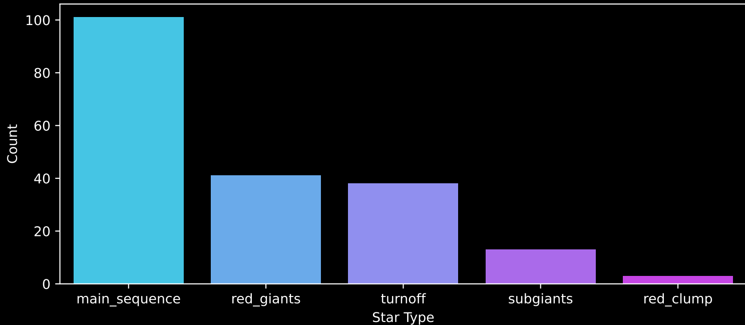
APOGEE DR17 Field: [176-27-O] Count plot of Star Type
