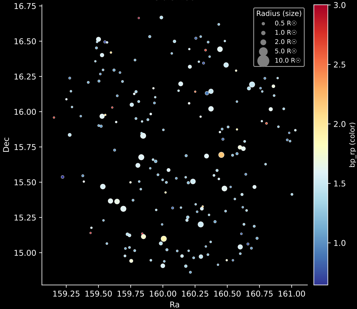
APOGEE DR17 Field: [176-27-O] Stars: 196
