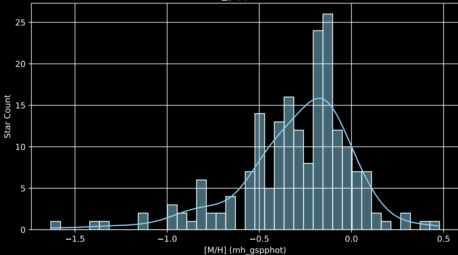
APOGEE DR17 Field: [176-27-O [M/H] (mh_gspphot) (n= 193)
