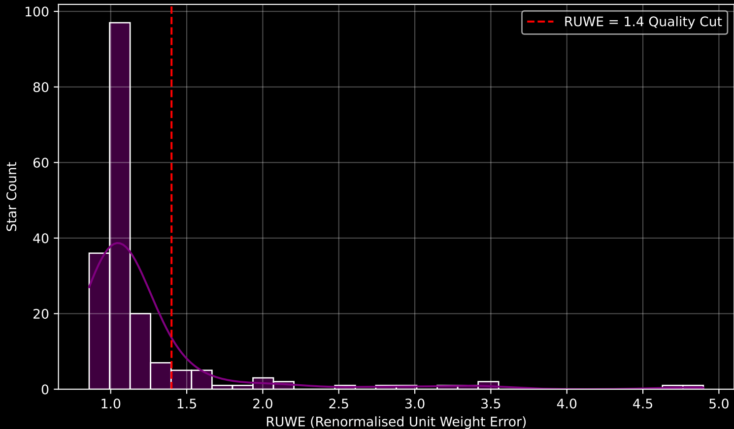
GAPOGEE DR17 Field [176-27-O] RUWE Distribution (n= 186)
